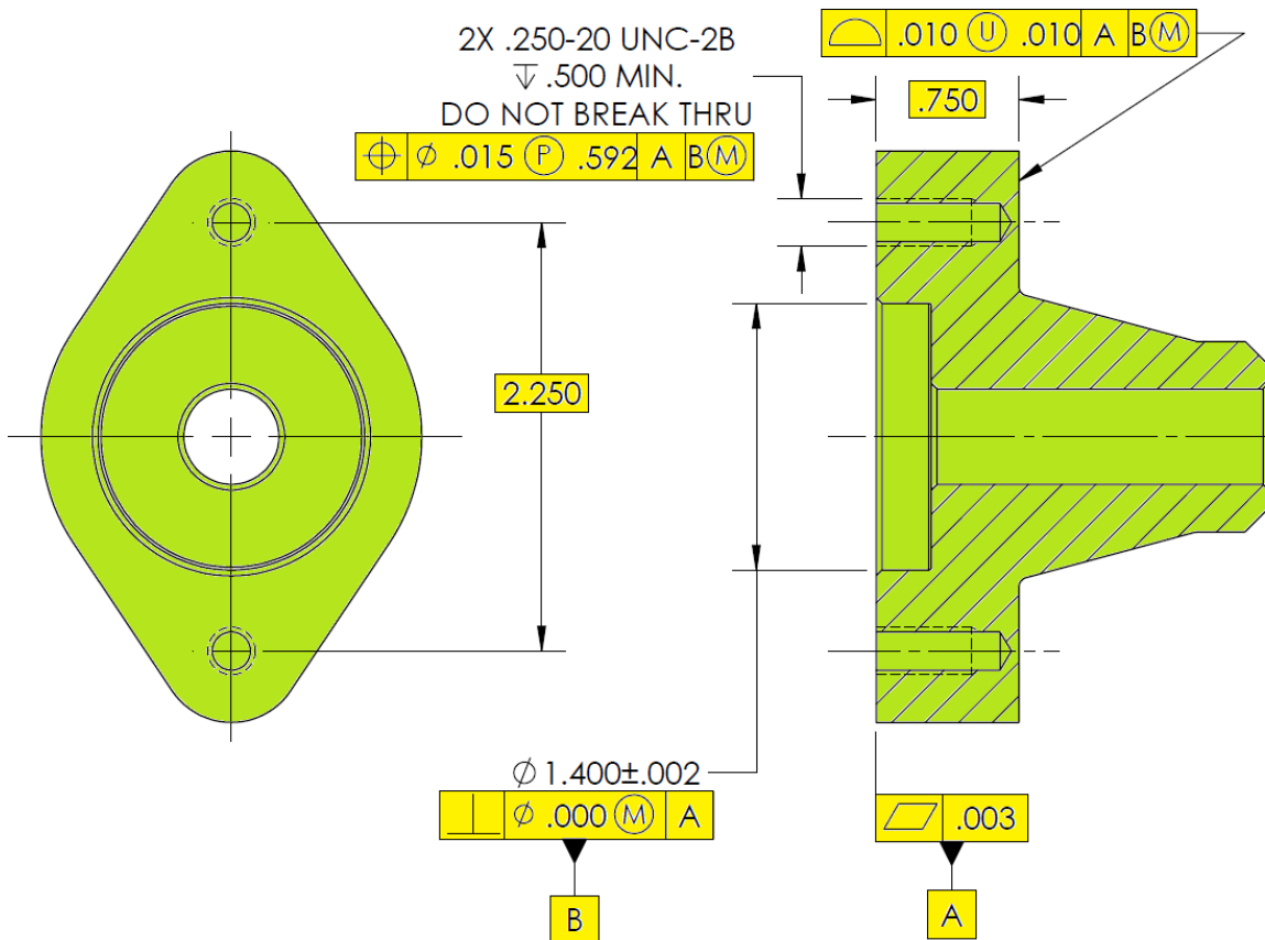
Figure 3, Female Weld Flange
