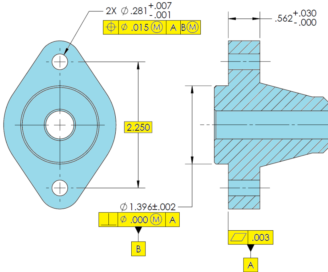
Figure 2, Male Weld Flange
